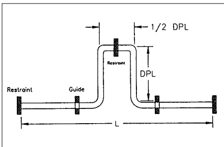
Expansion Loop
